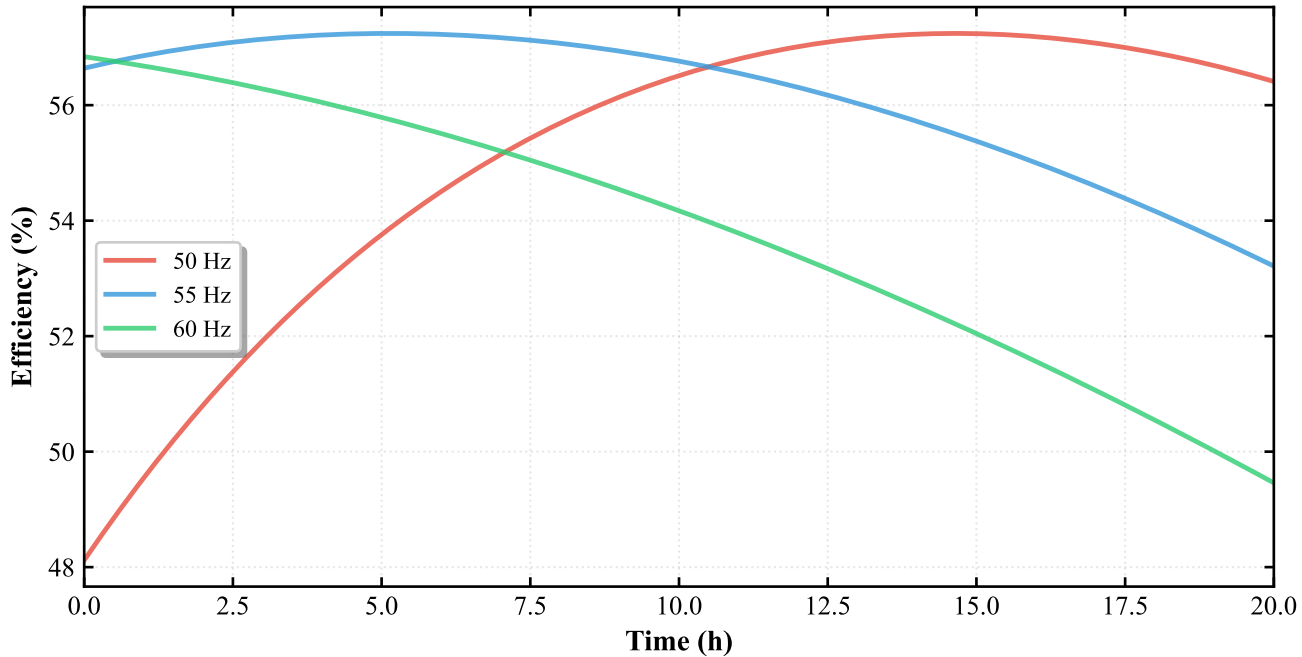
Efficiency vs Time at Constant Frequency (Head Decreasing)
