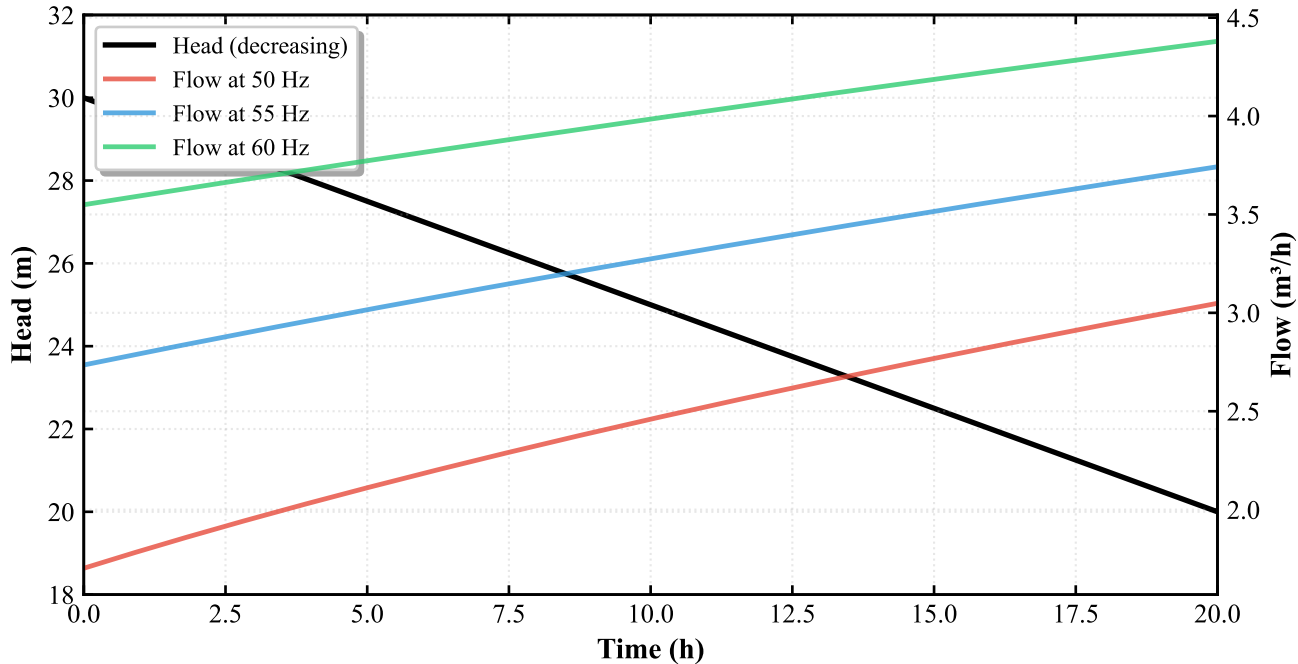
Flow Behavior vs Head Change at Constant Frequency
