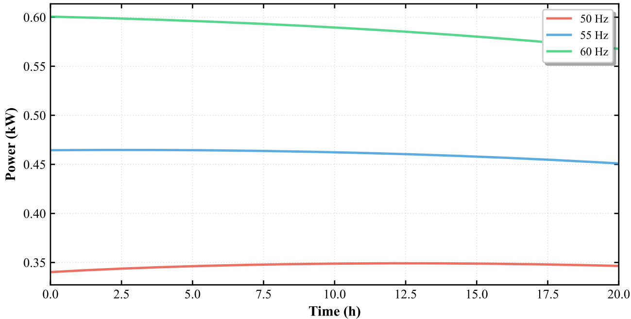
Power Consumption vs Time at Constant Frequency
