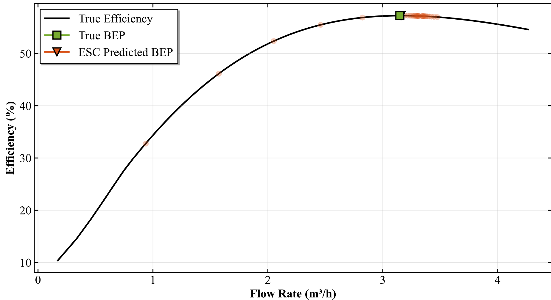
True vs Predicted Efficiency Curve (H = 30.0m)
