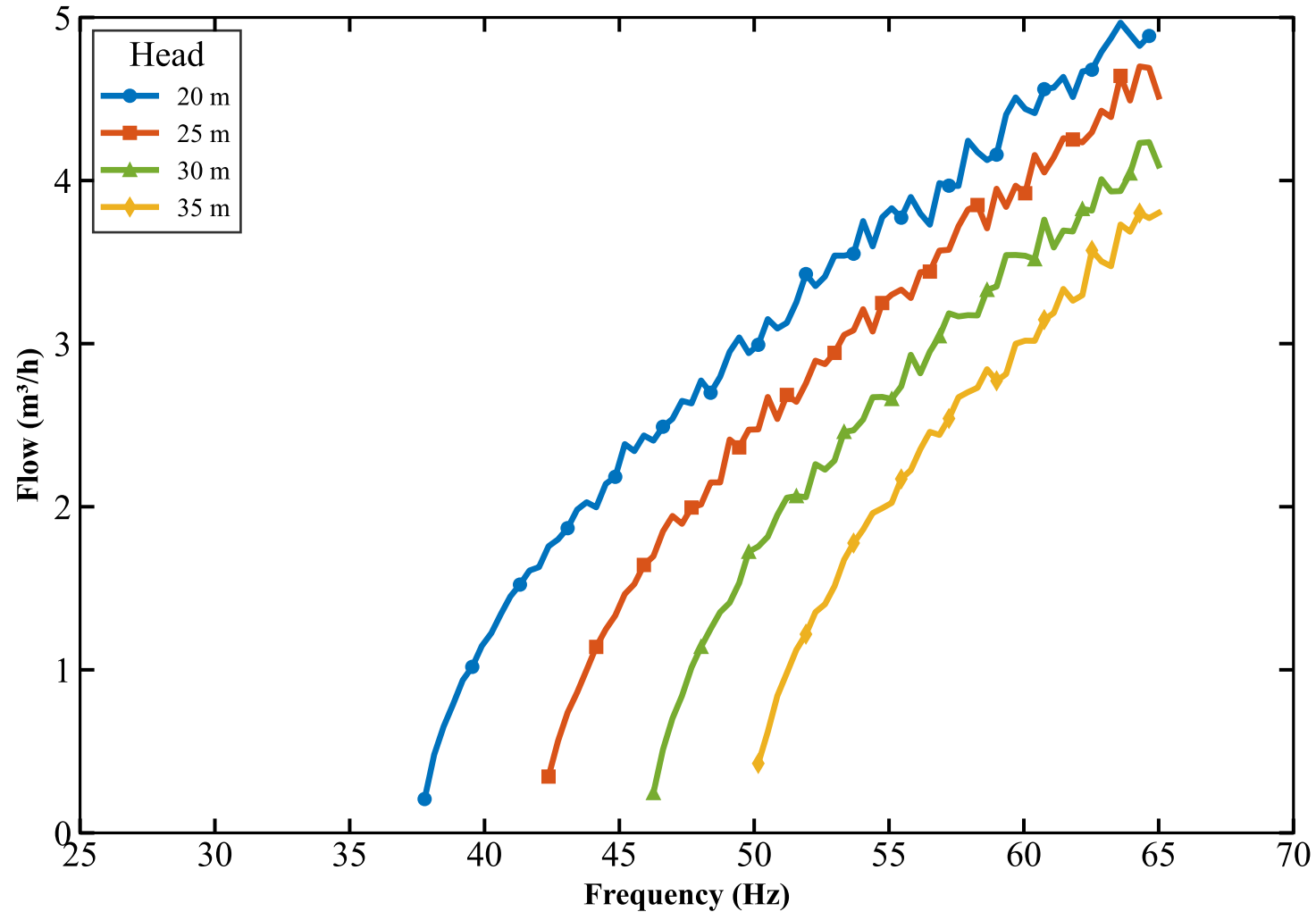
Flow vs Frequency at Constant Head
