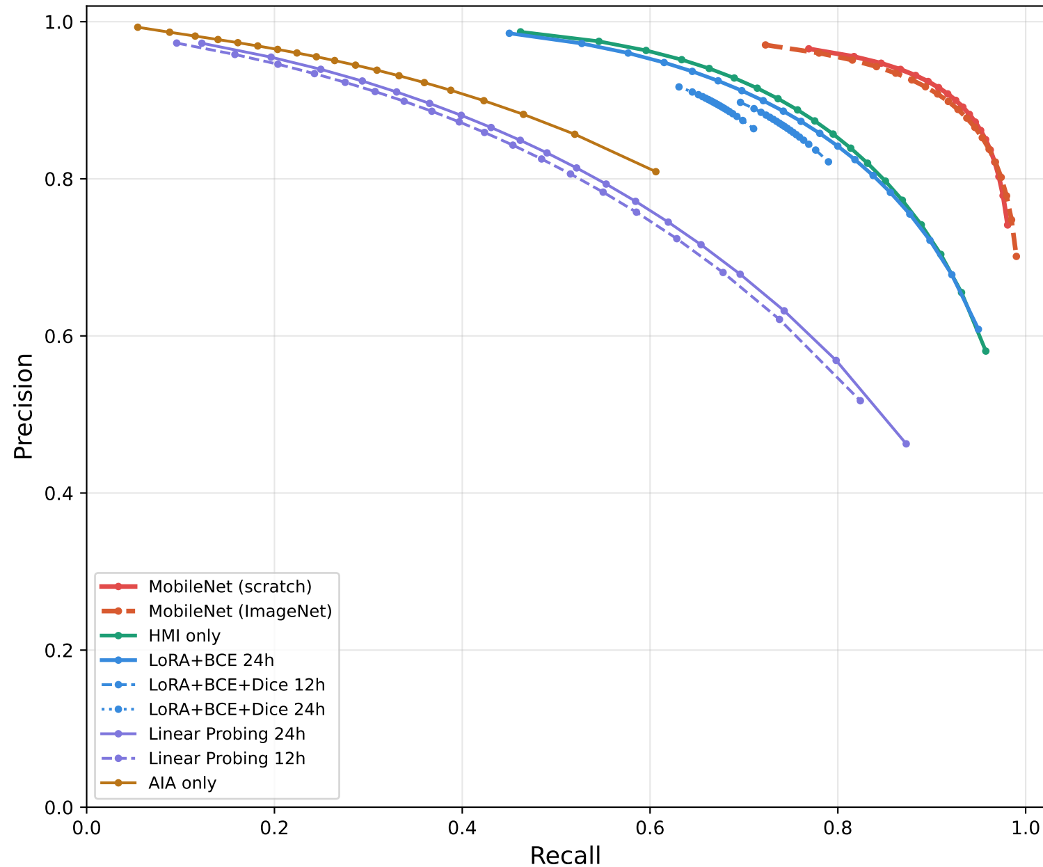
Precision-Recall Curve (Micro)
