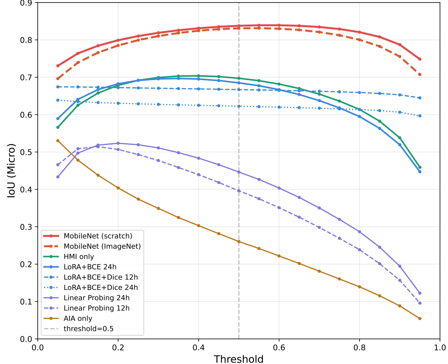
IoU vs Threshold
