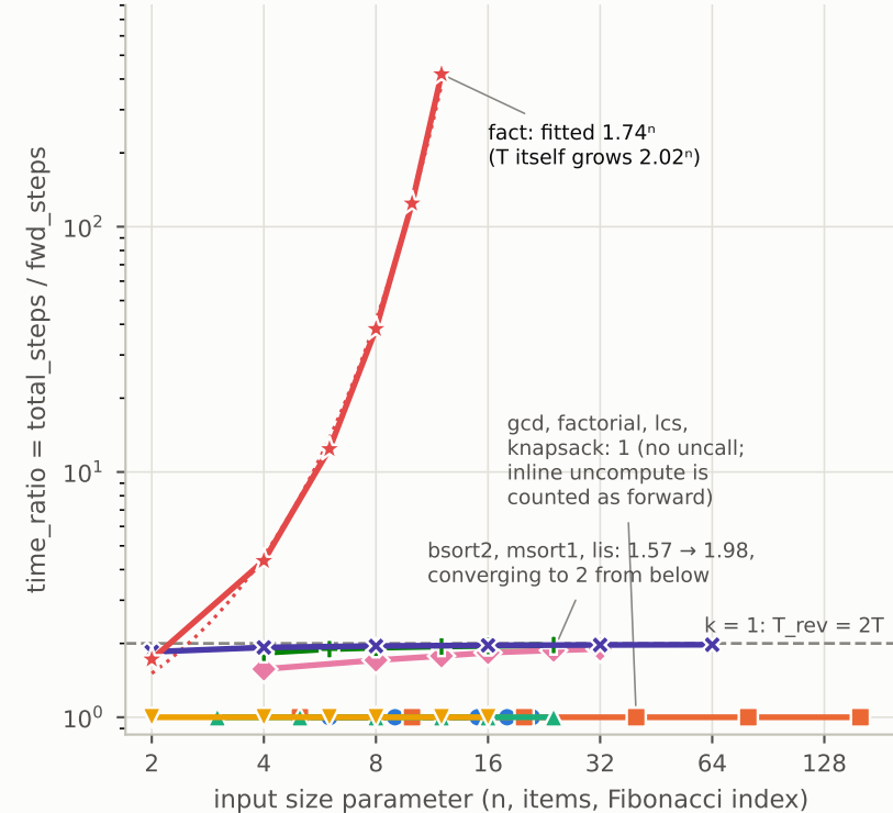
(c) time scaling, same programs
