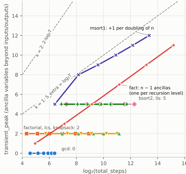
(b) space scaling, 8 programs \times 6 input sizes
