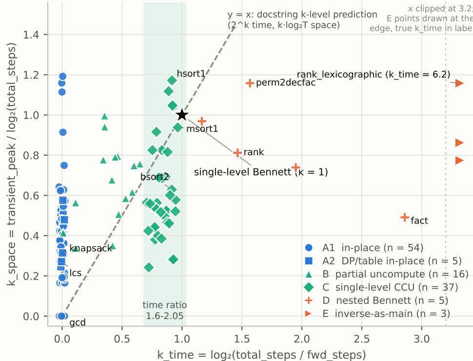
(a) 120 reversible-algorithms programs, by class
