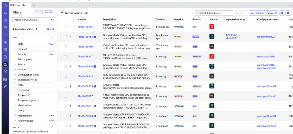
Figure 4. Express List page
