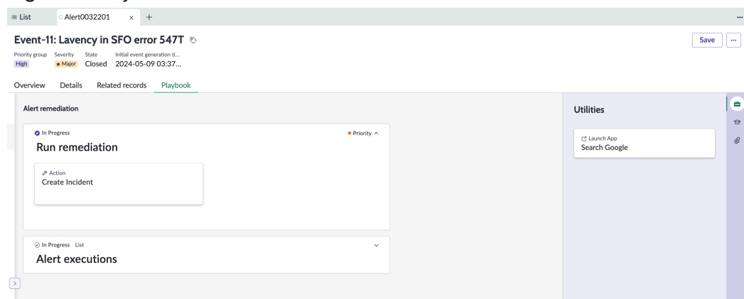
Figure 1. Playbook tab
