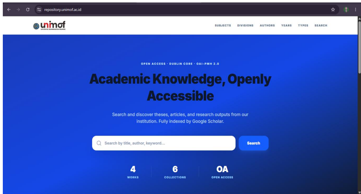
Gambar 7.4 Dashboard Repository
