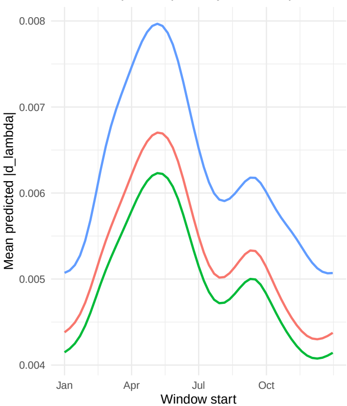
Seasonal profile (57-day windows)
