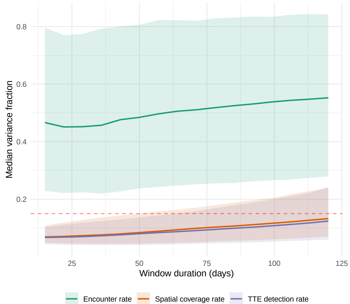
(b) Variance fraction by window duration
