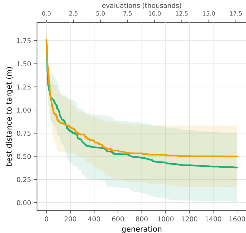
(a) Step size \times step direction
