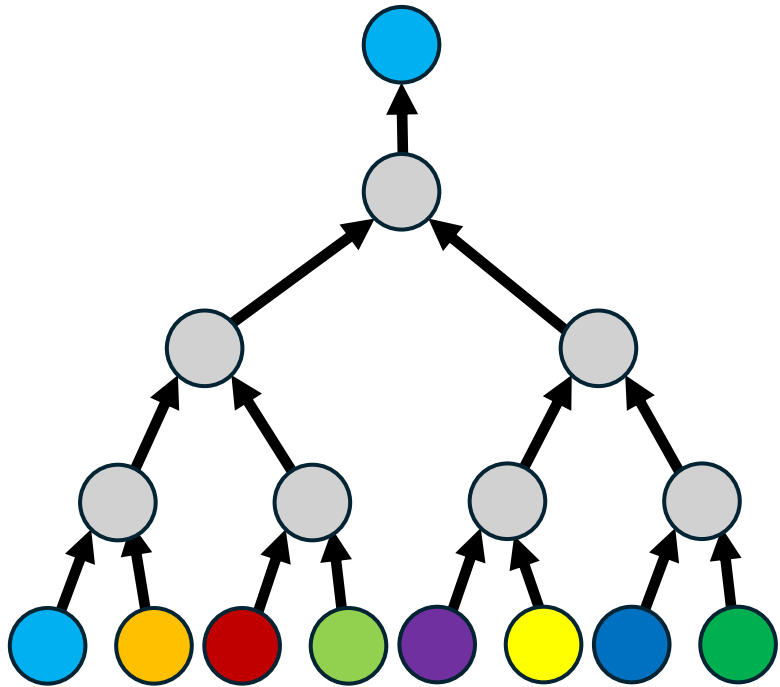
(a) Tree Neighbors-match
