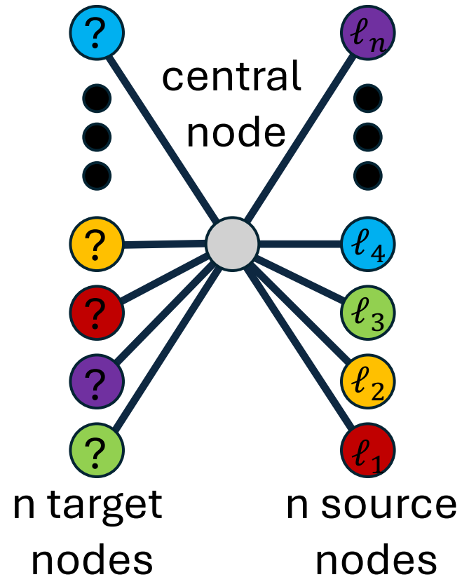
(c) Two-Radius ( k=1 )
