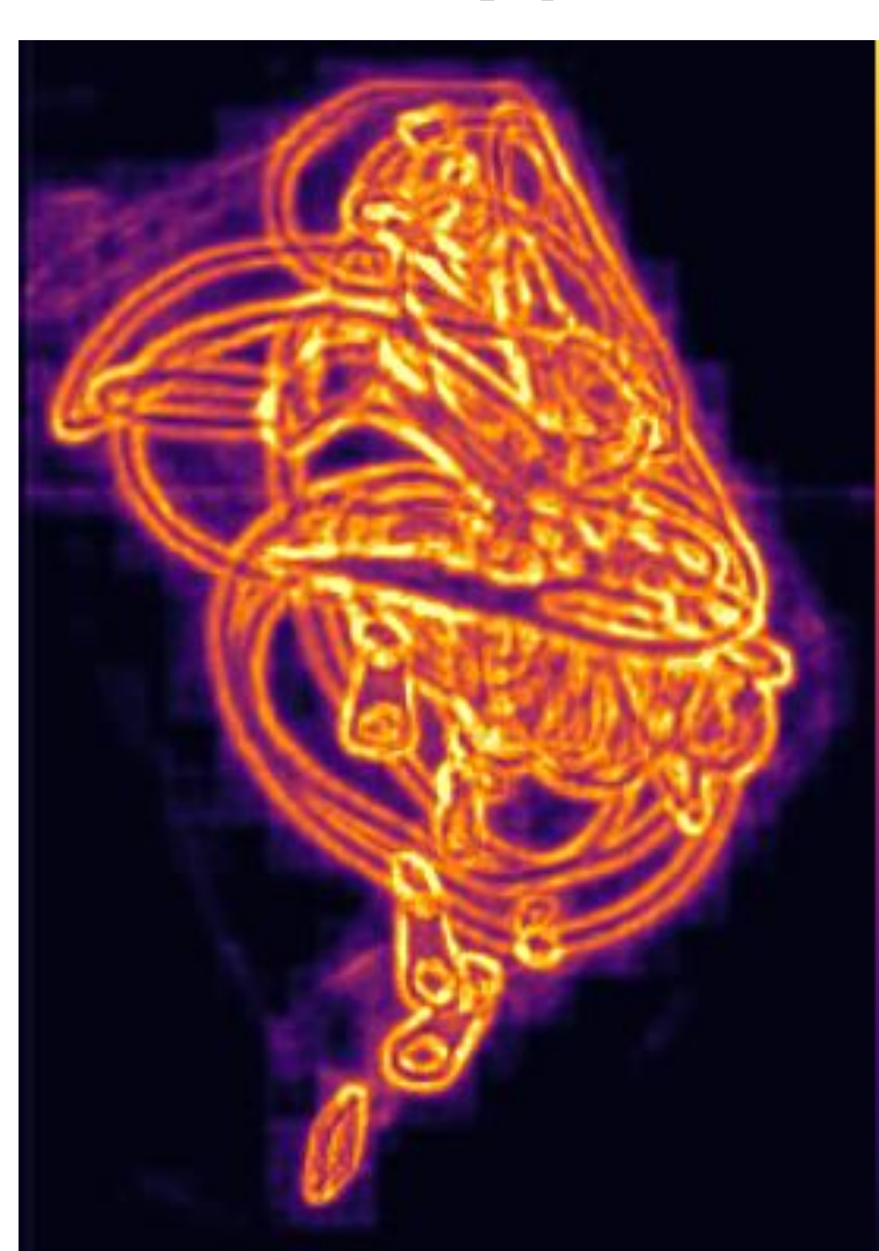
Boundary priors
