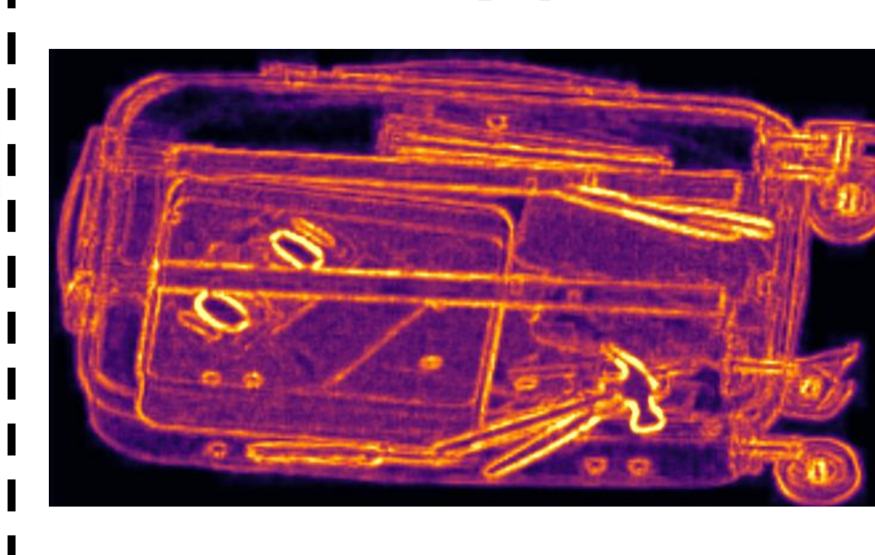
Boundary priors
