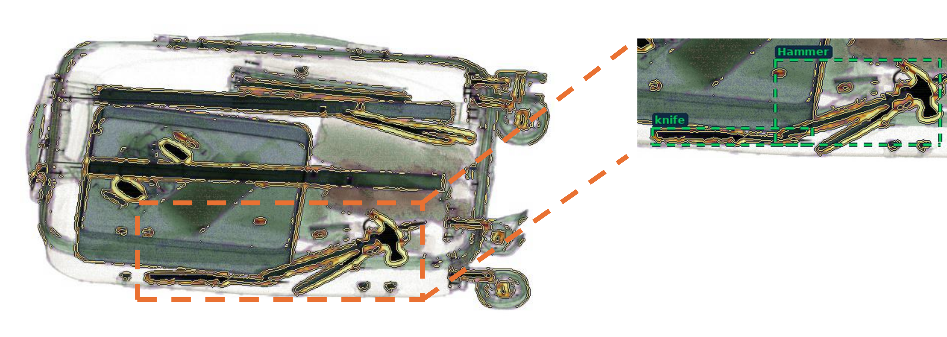
Residual predictions
