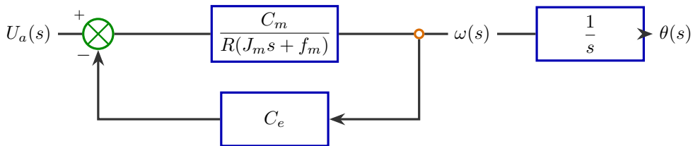
Equivalent reduced form
