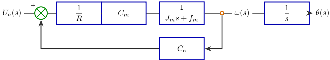
Original DC motor structure
