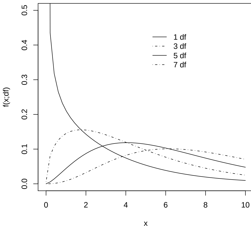
Non Central Chi-Square Densities with ncp = 1.5
