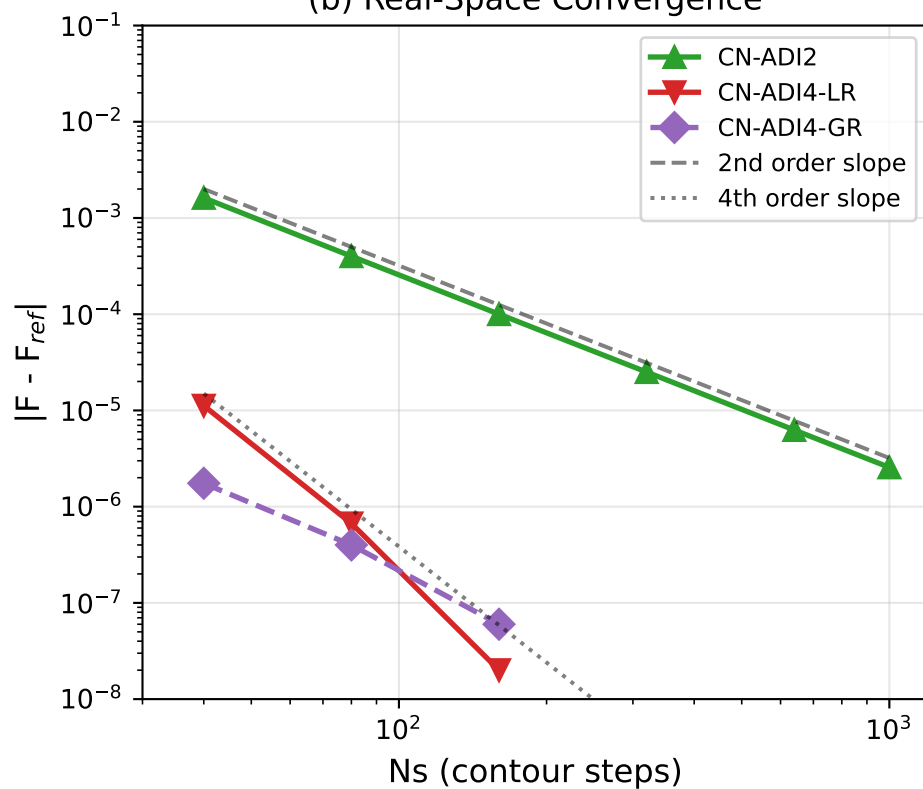
(b) Real-Space Convergence
