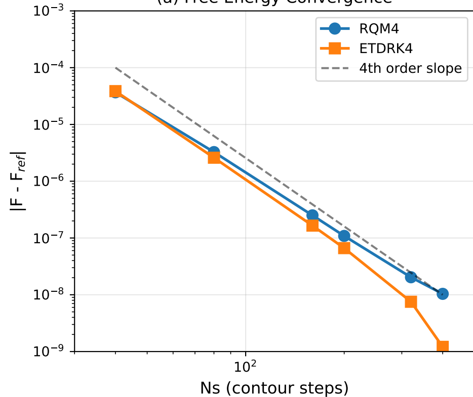
(a) Free Energy Convergence
