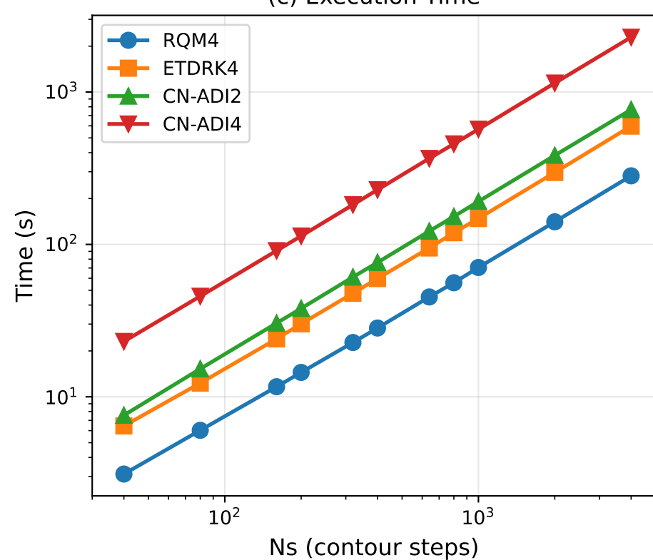
(c) Execution Time
