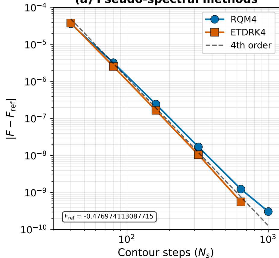
(a) Pseudo-spectral methods
