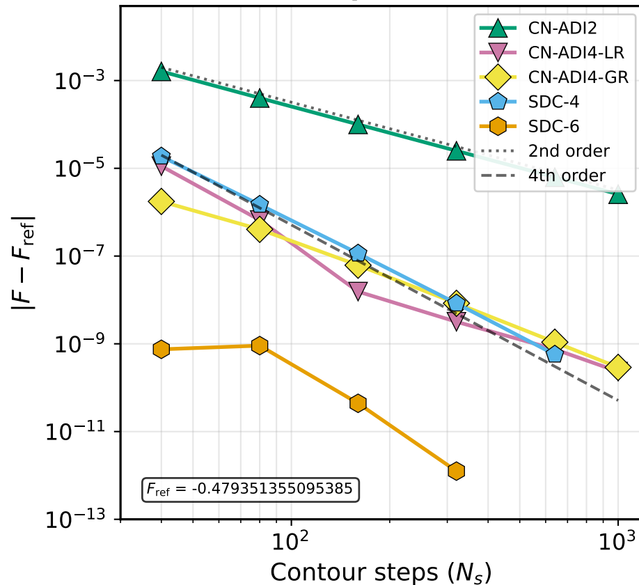
(b) Real-space methods
