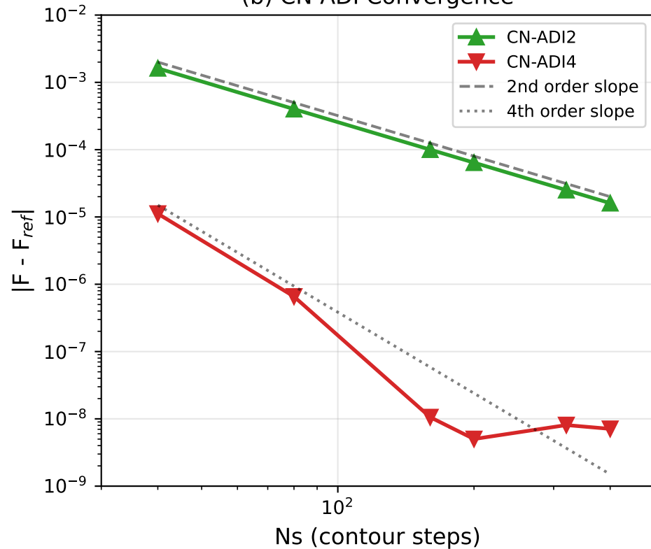
(b) CN-ADI Convergence
