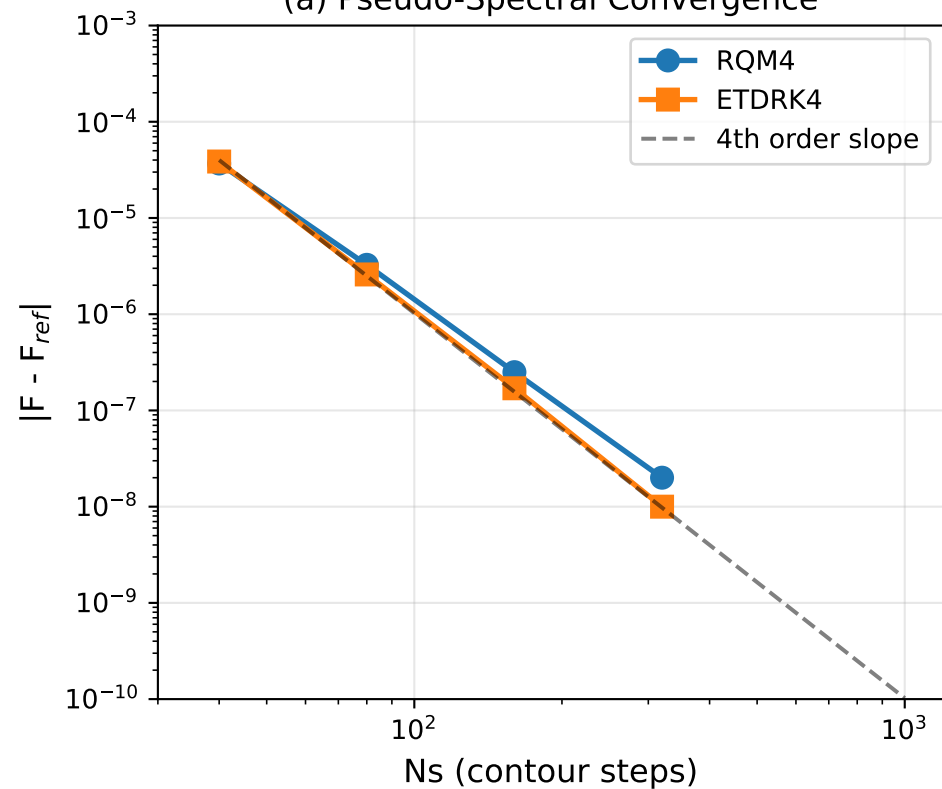
(a) Pseudo-Spectral Convergence
