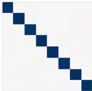
antmaze-giant
