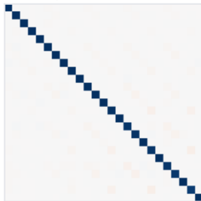
puzzle-4x4
