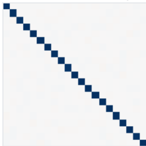
humanoidmaze-large
