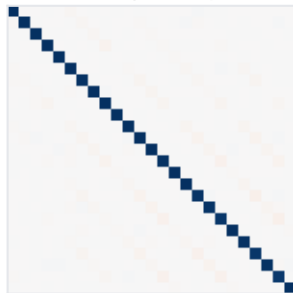
cube-quadraple
