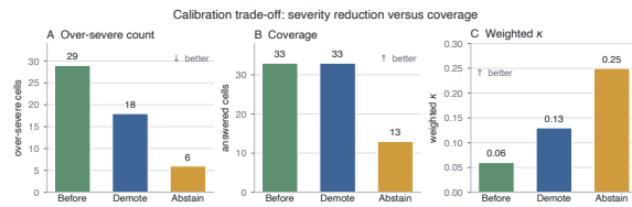
Figure 6: Calibration trade-off: severity reduction versus coverage against the adjudicated human gold. Demoting weak-retrieval high s to medium preserves coverage (33 answered) while cutting over-severe judgments from 29 to 18; abstaining gives the strongest correction (over-severe 6, weighted \kappa 0.25) but leaves only 13 answered cells. Calibration corrects severity bias; the remaining bottleneck is evidence grounding, not severity thresholding alone.
