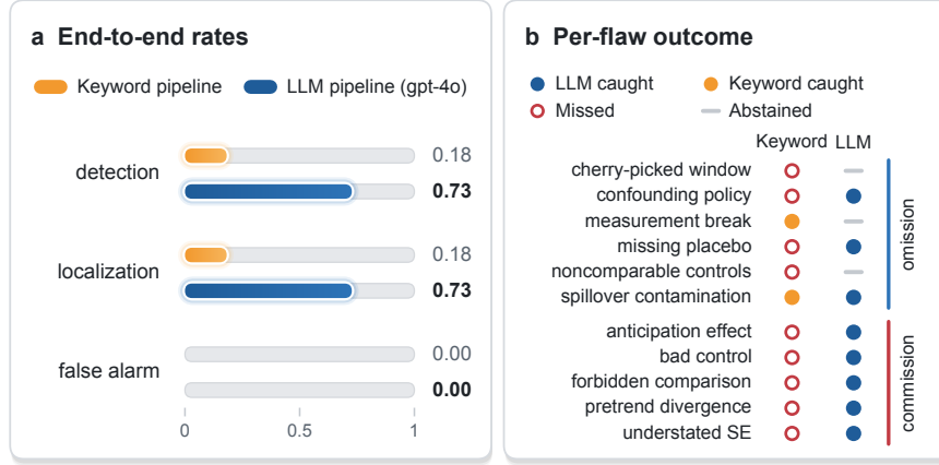
Figure 3: Keyword pipeline vs. LLM evidence-adequacy pipeline ( n=11 flaws, realistic injection). (a) End to end, the LLM pipeline raises detection and localization 0.182 \rightarrow 0.727 with false alarm 0 (the two pipelines retrieve evidence differently; Appendix K holds it fixed). (b) Per-flaw caught/missed: the keyword baseline is blind to every commission-type flaw , all of which the LLM catches; the LLM’s three misses are omissions on which it abstains. Table 2 reports the harder 33-variant benchmark.
