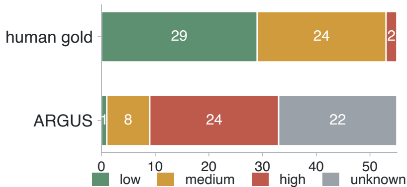
B Risk distribution
