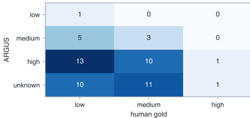
D Confusion matrix
