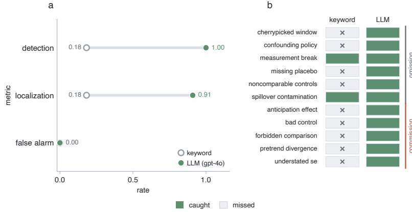
Figure 3: Keyword baseline vs. LLM evidence-adequacy assessor ( n=11 flaws, realistic injection). (a) Swapping only the assessment policy—same retrieved evidence—recovers detection 0.182 \rightarrow 1.000 and localization 0.182 \rightarrow 0.909 ; false alarm 0. (b) Per-flaw caught/missed: the keyword baseline is blind to every commission-type flaw , all of which the LLM catches.
