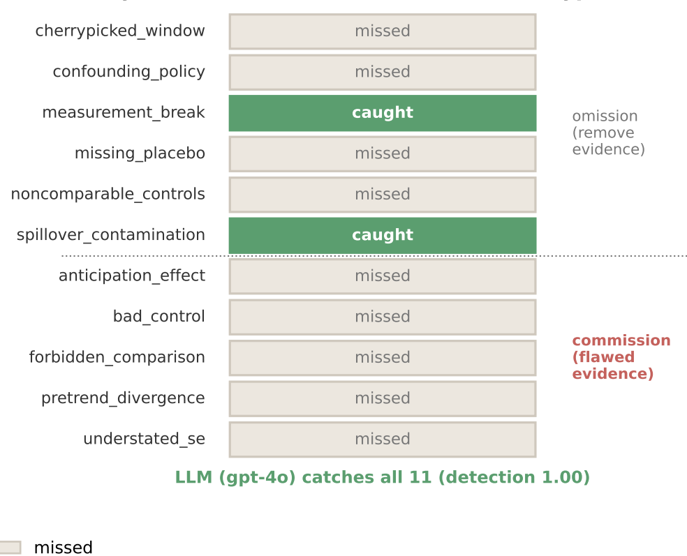
B Keyword baseline: blind to commission-type flaws
