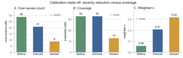
Figure 6: Calibration trade-off: severity reduction versus coverage against the adjudicated human gold, for the weak-retrieval rule alone (in-sample; Table 14 adds the exploratory four-rule set). Demoting weak-retrieval high s to medium preserves coverage (33 answered) while cutting over-severe judgments from 29 to 21; abstaining leaves fewer over-severe cells (9) and a higher weighted \kappa (0.32) only by discarding 20 answers, and fixes none of them. Calibration reduces severity bias; the remaining bottleneck is evidence grounding, not severity thresholding alone.
