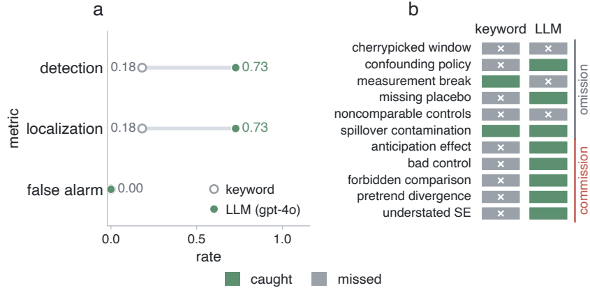
Figure 3: Keyword baseline vs. LLM evidence-adequacy assessor ( n=11 flaws, realistic injection). (a) End to end, the LLM pipeline raises detection and localization 0.182 \rightarrow 0.727 with false alarm 0 (the two pipelines retrieve evidence differently; Appendix K holds it fixed). (b) Per-flaw caught/missed: the keyword baseline is blind to every commission-type flaw , all of which the LLM catches; the LLM’s three misses are omissions on which it abstains. Table 2 reports the harder 33-variant benchmark.
