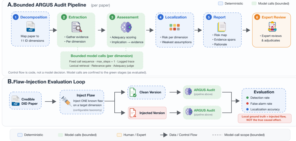
Figure 2: ARGUS architecture. The top band is the audit pipeline, a fixed deterministic sequence; model calls are confined to two stages (extraction and assessment). As evaluated, these resolve per dimension to a fixed call sequence (lexical retrieval, one relevance-gate call, one adequacy call) with a step budget of one and a logged trace; the designed tools figure_parse and policy_lookup are not exercised (§3.2). The bottom band shows the flaw-injection evaluation loop, which injects one known flaw, audits the clean and injected versions, and scores detection, false alarm, and localization against the injected flaw as local ground truth, never against the unobserved true effect.
