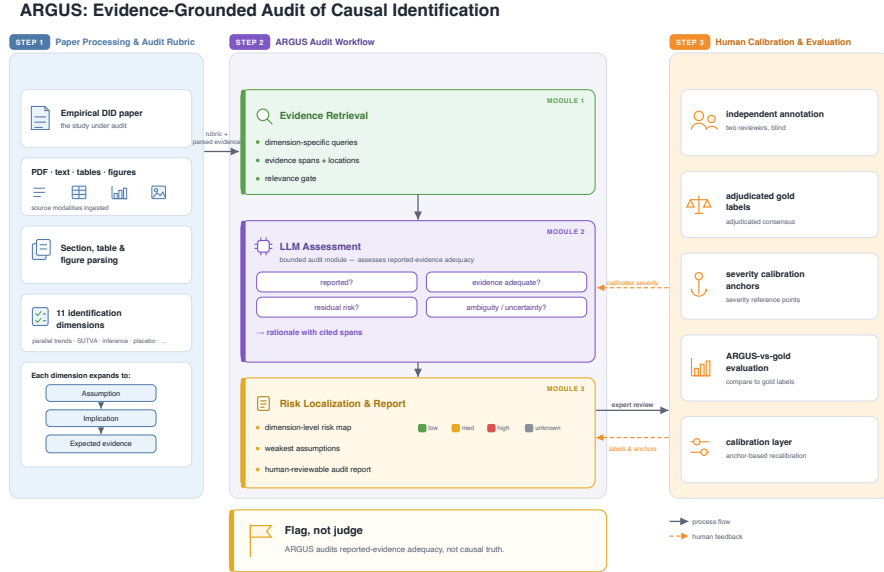
Fig. 1. Overview of ARGUS. Step 1 converts an empirical DID paper into an auditable structure using an 11-dimension identification rubric. Step 2 retrieves dimension-specific evidence, assesses reported-evidence adequacy with a bounded LLM audit module, and localizes risk in a human-reviewable report. Step 3 uses expert annotation and adjudicated gold labels to evaluate and calibrate audit severity. ARGUS flags dimensions for expert review; it does not adjudicate causal truth.
