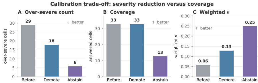
Fig. 6. Calibration trade-off: severity reduction versus coverage. Calibration trade-off against adjudicated human gold. Demoting weak-retrieval high-risk judgments to medium preserves coverage while reducing over-severity. Abstaining instead gives the strongest severity correction and highest weighted agreement, but sharply reduces coverage. This shows that human-gold calibration can correct severity bias, while the remaining bottleneck is evidence grounding rather than severity thresholding alone.
