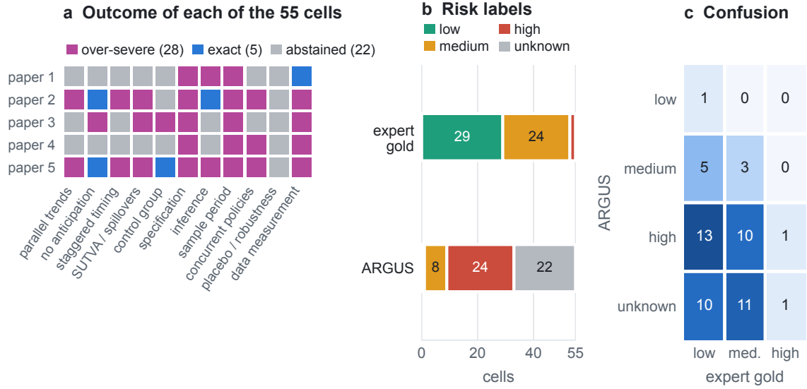
Figure 4: ARGUS-LLM versus the adjudicated expert gold on the 55 pilot cells (frozen protocol). (a) Every cell, five papers by eleven dimensions, coloured by outcome: ARGUS abstains on 22 and, of the 33 it answers, is more severe than the gold on 28, matches it on 5, and is less severe on none. (b) Distribution of risk labels in the gold and in ARGUS’s output. (c) ARGUS-by-gold confusion matrix (counts).
