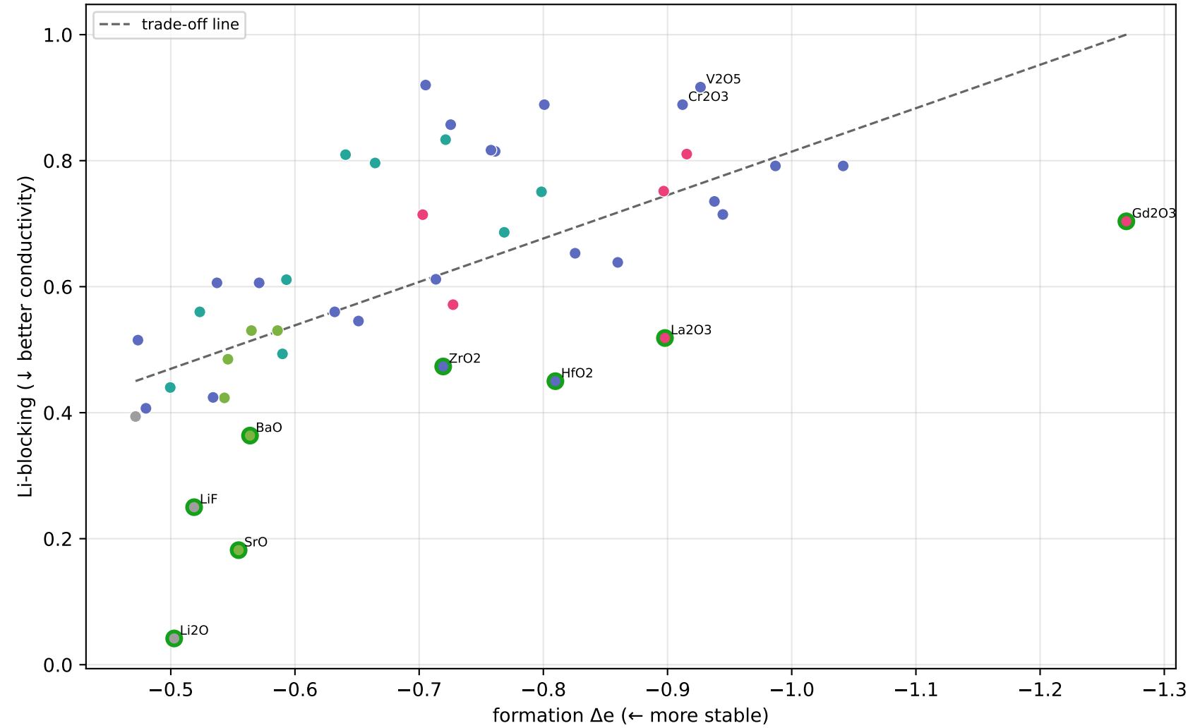
(D) Bulk sweet-spot — green ring = escaper (stable + low-block) ideal bulk dopant = lower-left, below the line
