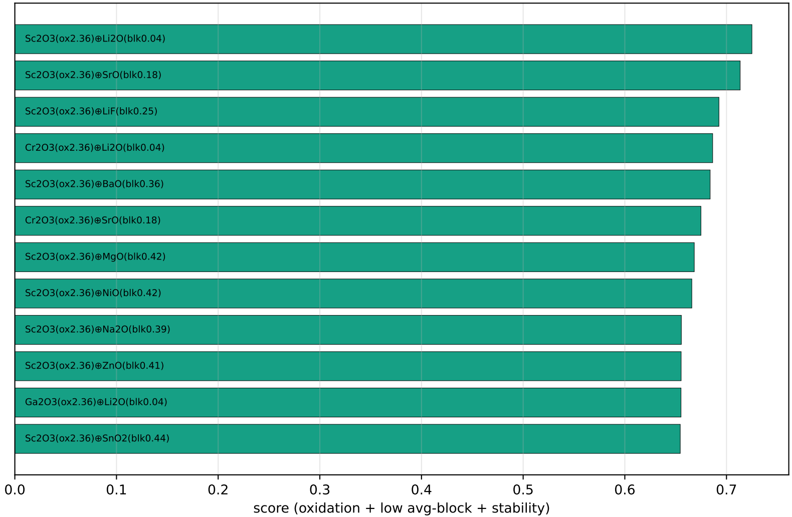
(C) STABILIZER ⊕ CONDUCTOR co-doping (keep ox, recover \sigma_{\text{Li}} )
