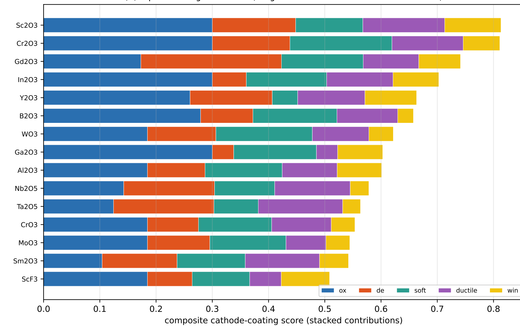
(C) Top-15 coating candidates (weights: ox.30 de.25 soft.20 duct.15 win.10)
