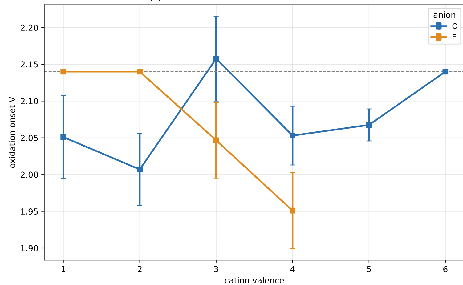
(D) Regression w/ interaction term (* = |t| > 2 ) valence:isF = interaction strength
