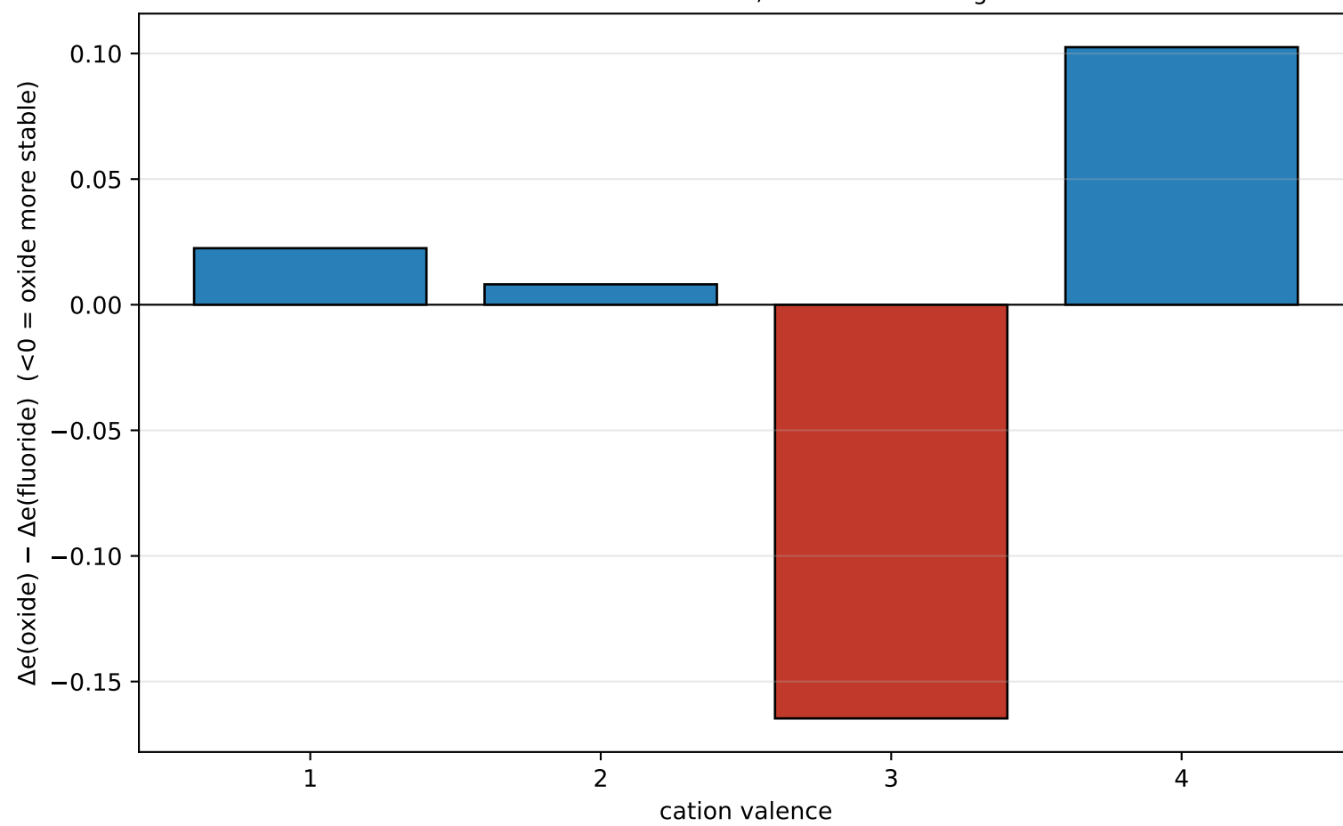
(C) Anion effect is NOT constant across valence = the interaction val 3: oxide much more stable; val 4: fluoride edges ahead
