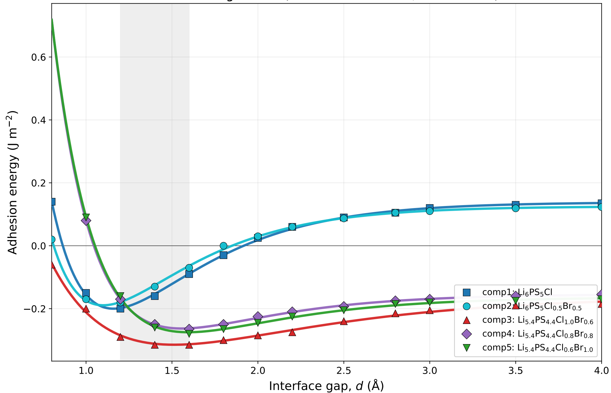
UMA binding curves (Morse-fit smoothed, R = +0.931 )
