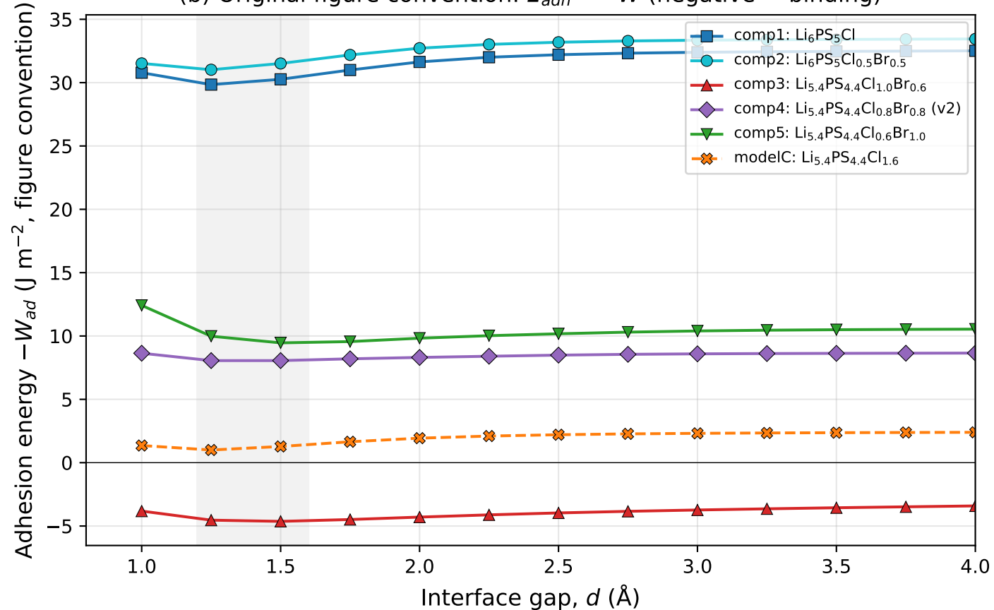
(b) Original figure convention: E_{adh} = -W (negative = binding)
