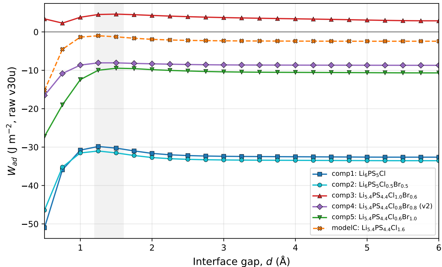
(a) Raw W_{ad} from v30u UMA Z-scan R(W_{max} \text{ vs paper exp}) = +0.964
