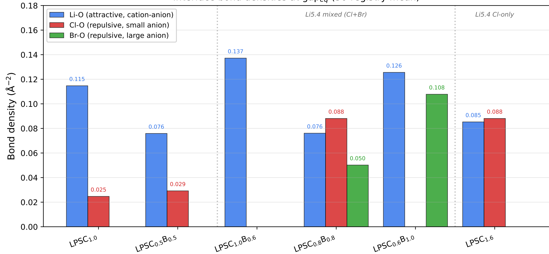
Interface bond densities at \text{gap}_{eq} (36-registry mean)
