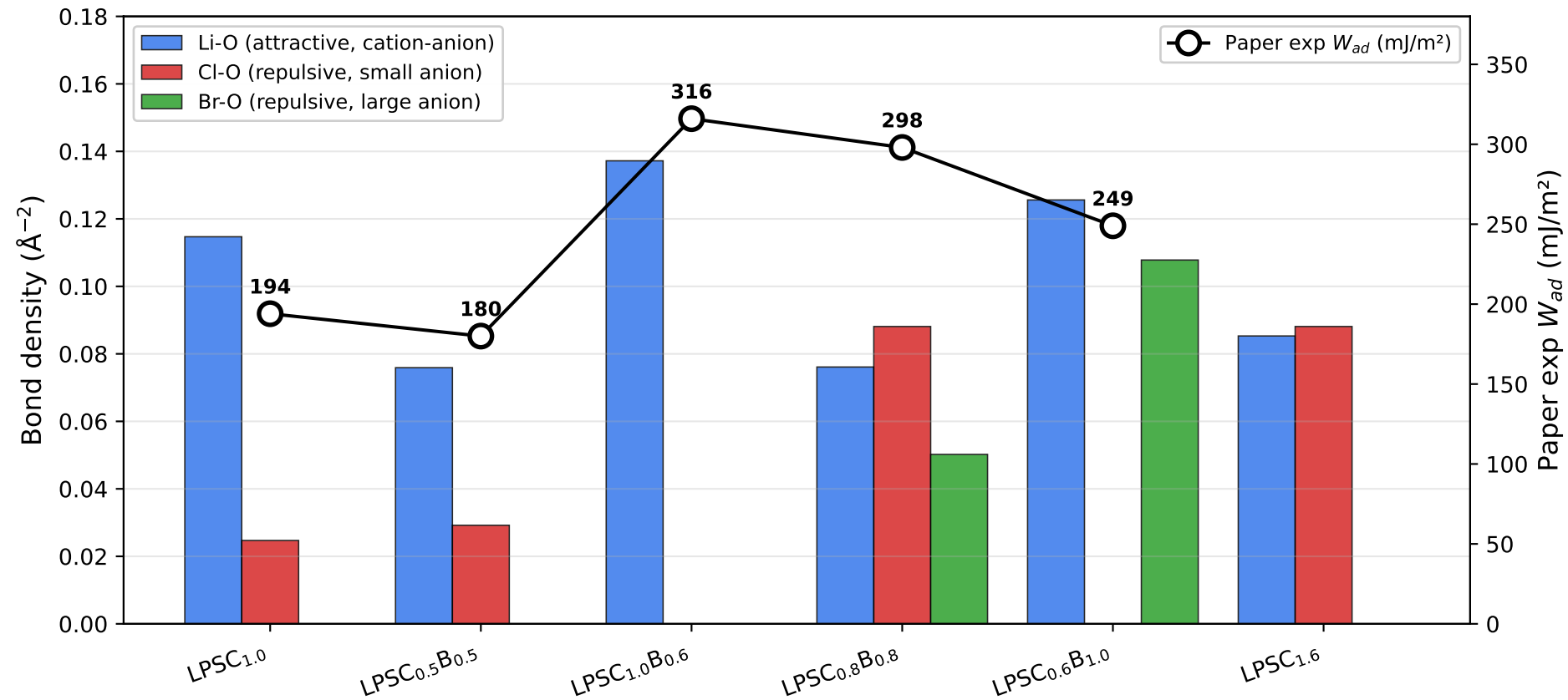
Interface bond densities and experimental adhesion
