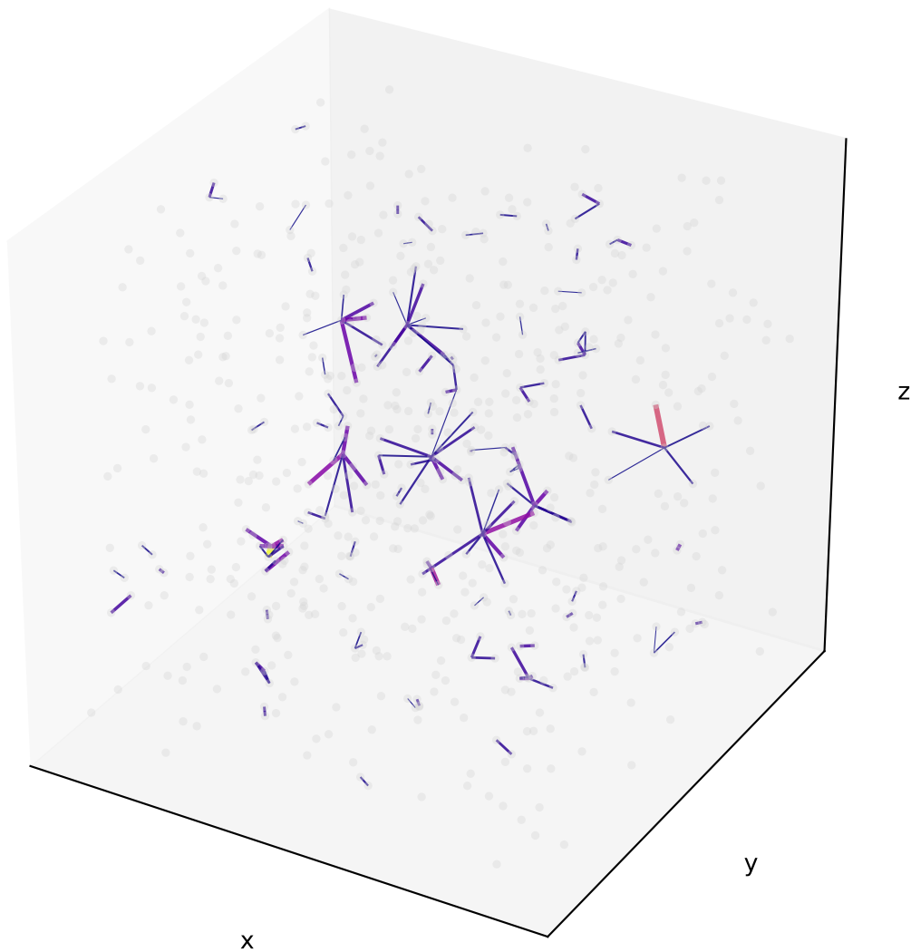
(c) Equivalent Kirchhoff resistor network (edge thickness \propto 1/R ; colour: low \rightarrow high conductance)
