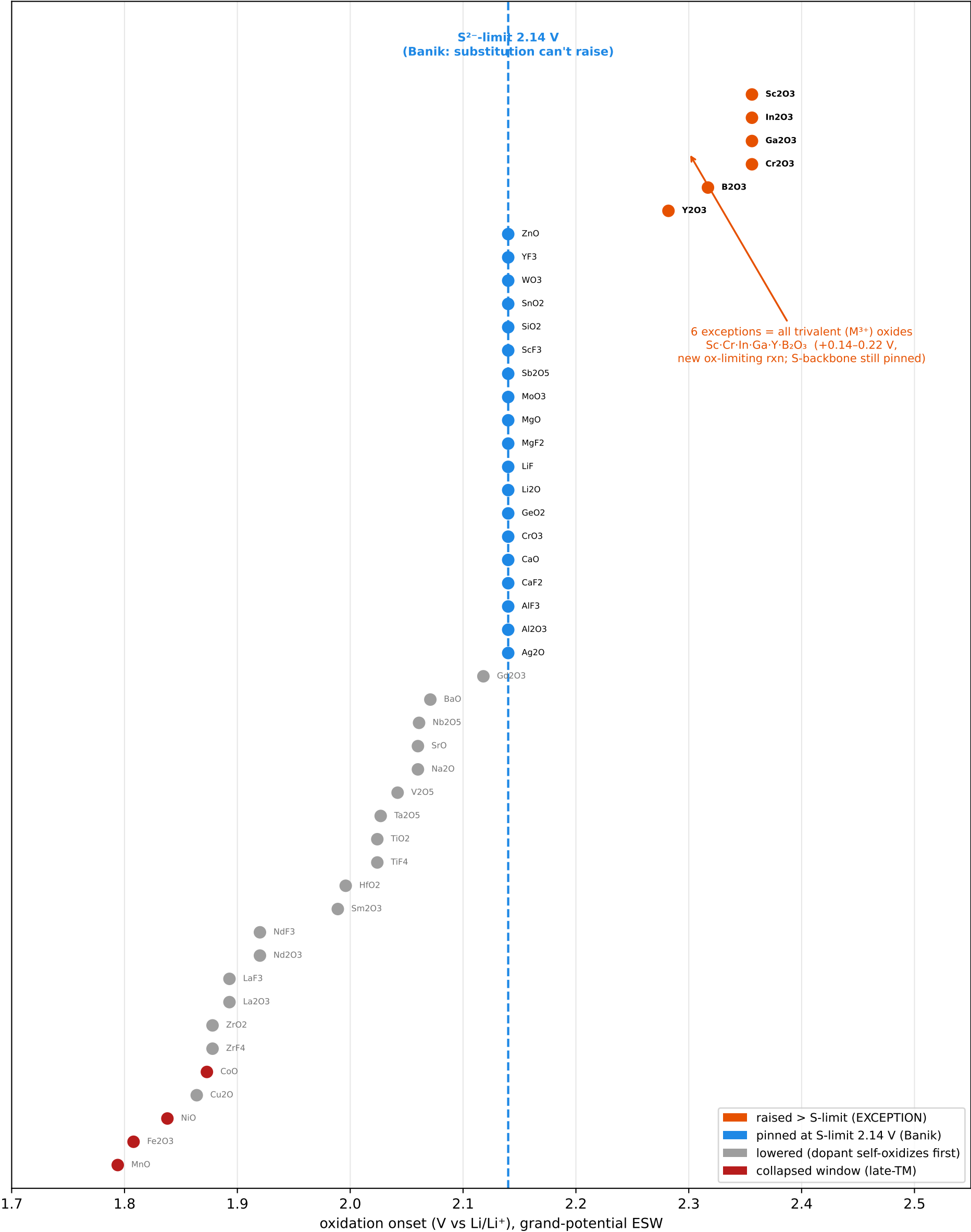
Cascade oxidation onset vs the Banik S-pin thesis pinned 19 · raised 6 (M 3+ oxides) · lowered 18 · collapsed 4 (of 47)
