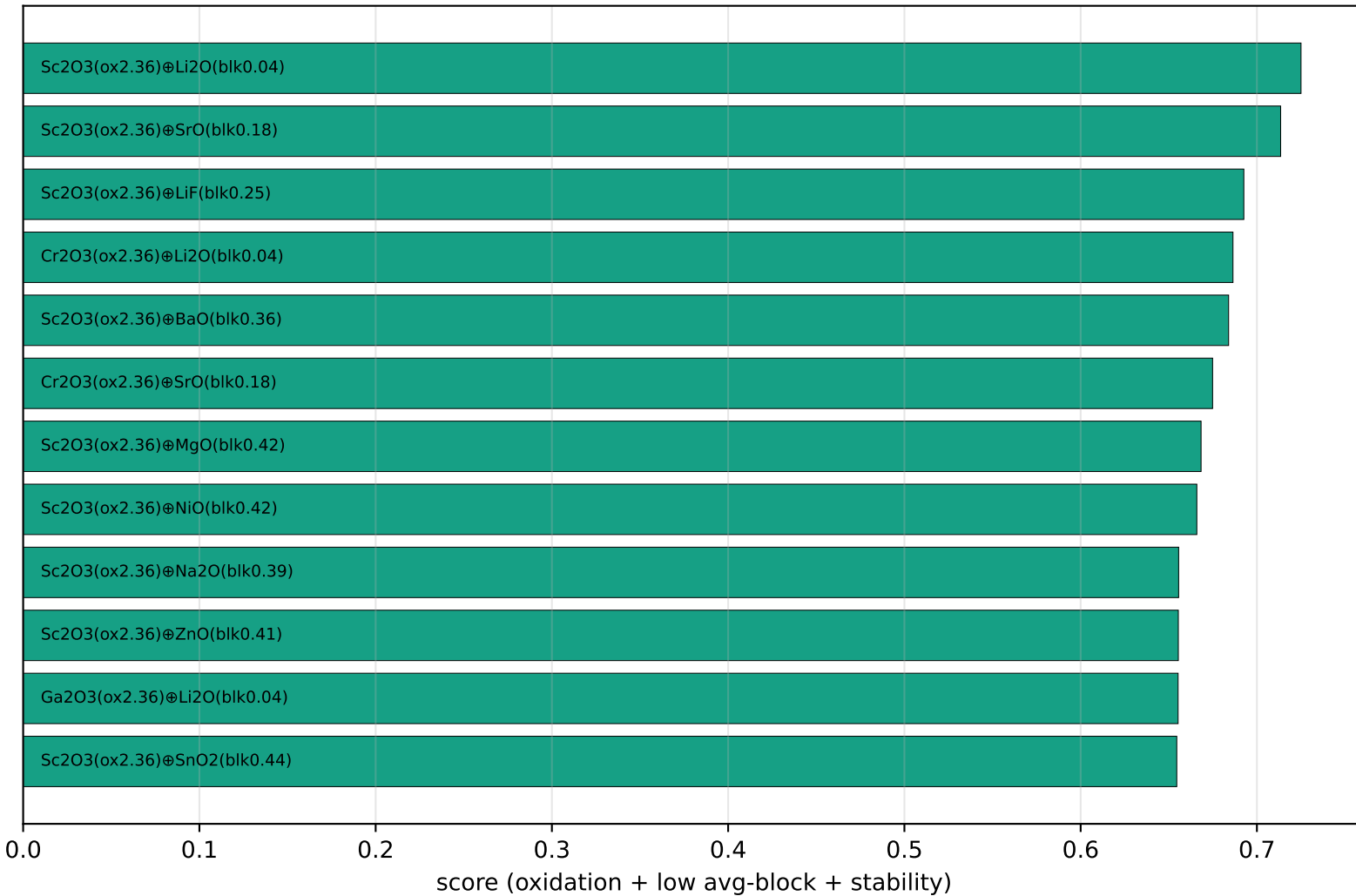
(C) STABILIZER @ CONDUCTOR co-doping (keep ox, recover \sigma_{\text{Li}} )
