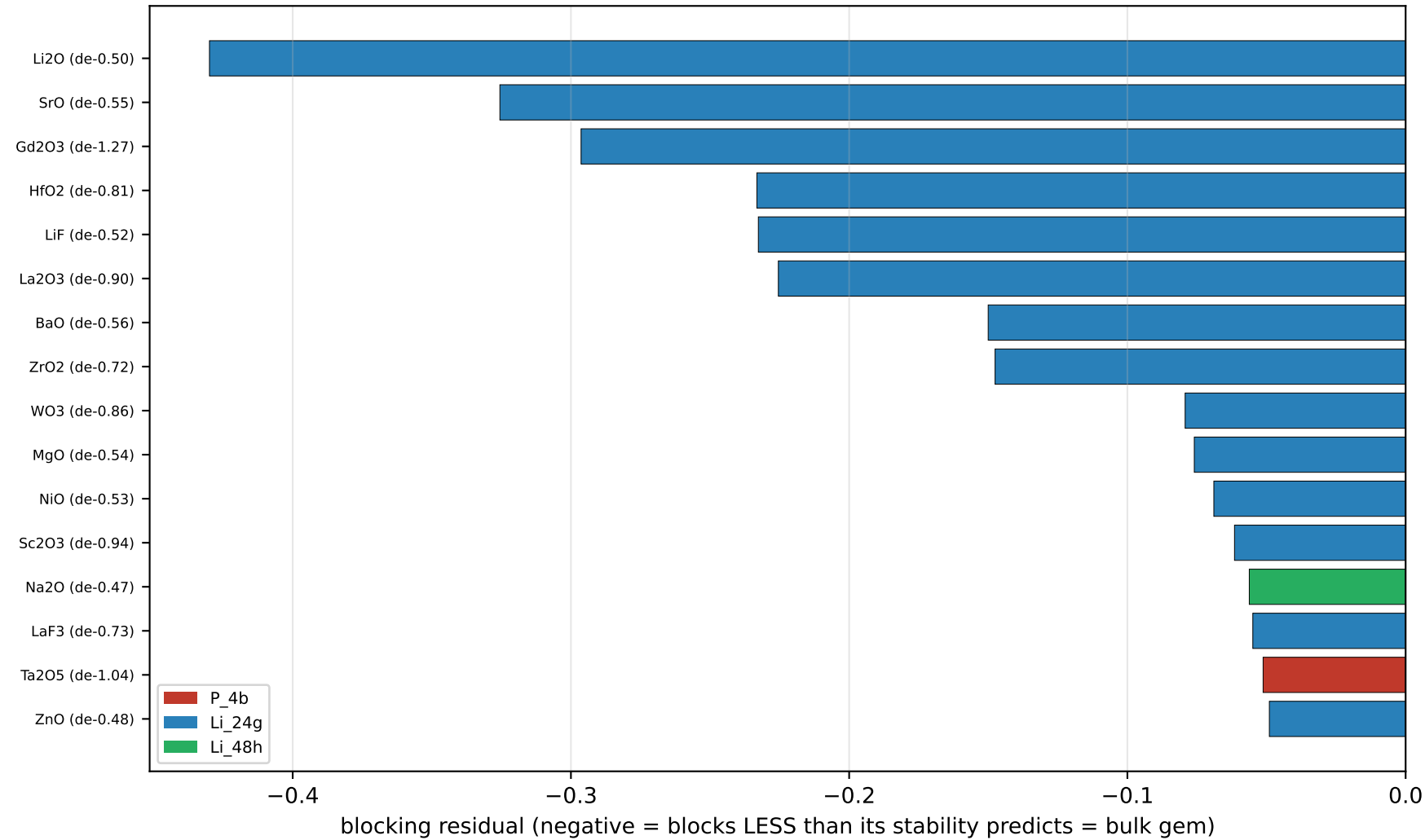
(A) Trade-off ESCAPERS — stable AND low-blocking (bulk-dopant gems)
