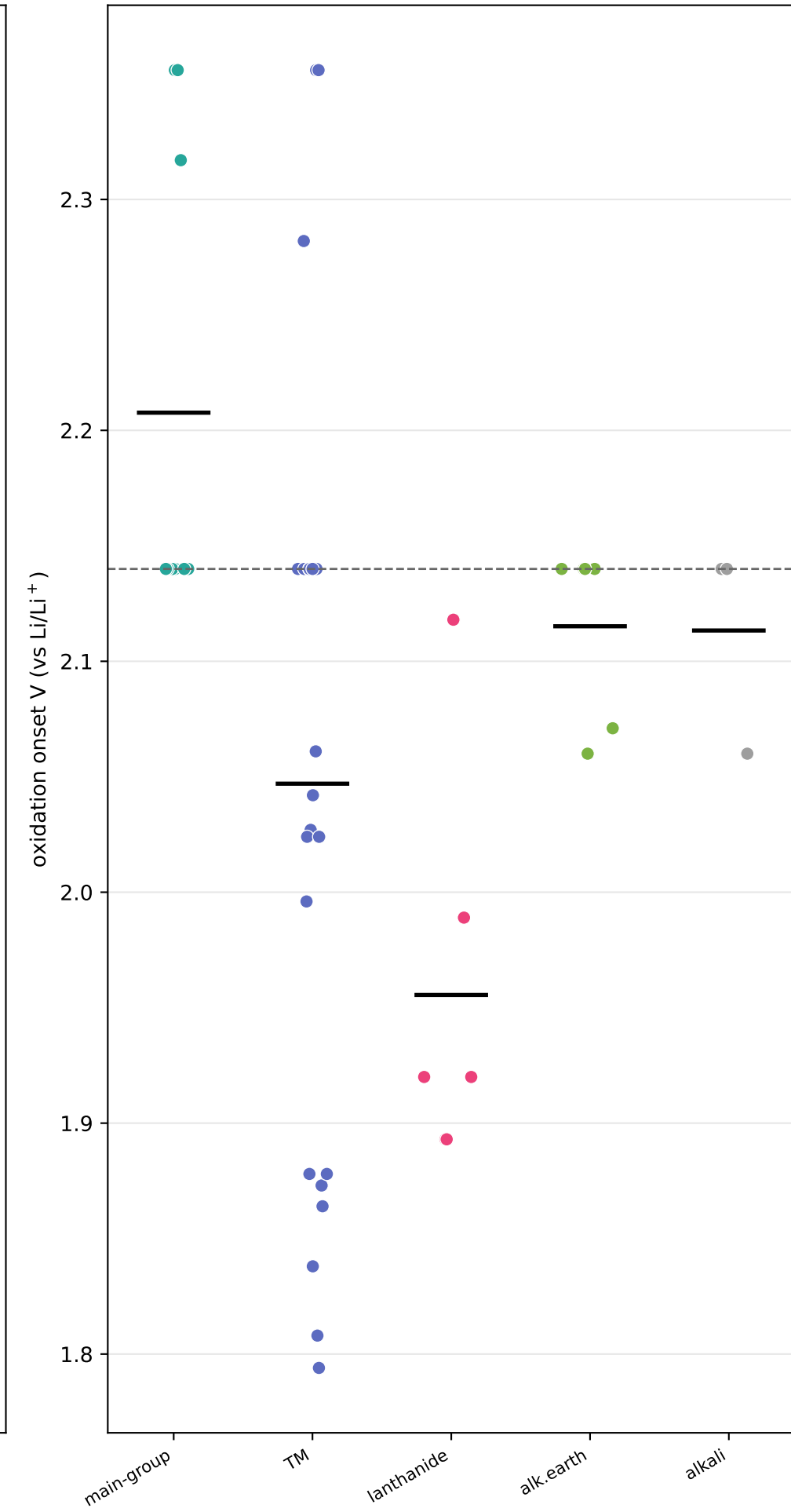
(B) Oxidation onset by cation group main-group/early-TM push it up; late-TM collapse it
