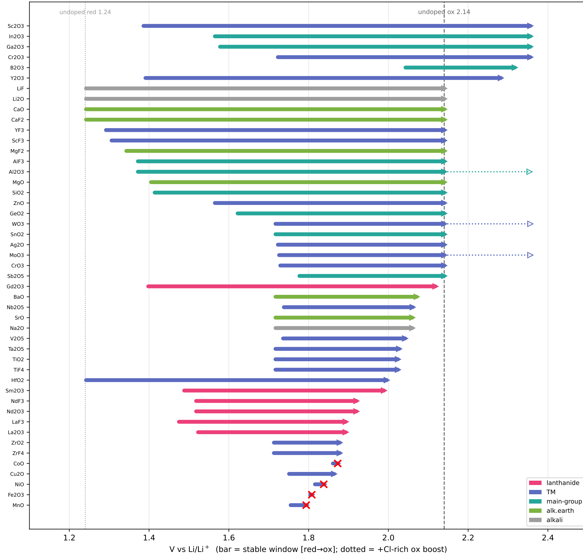
(A) Grand-potential stability window per dopant (sorted by ox onset) red x = collapsed window (M-redox eats it: Fe/Co/Ni/Mn)
