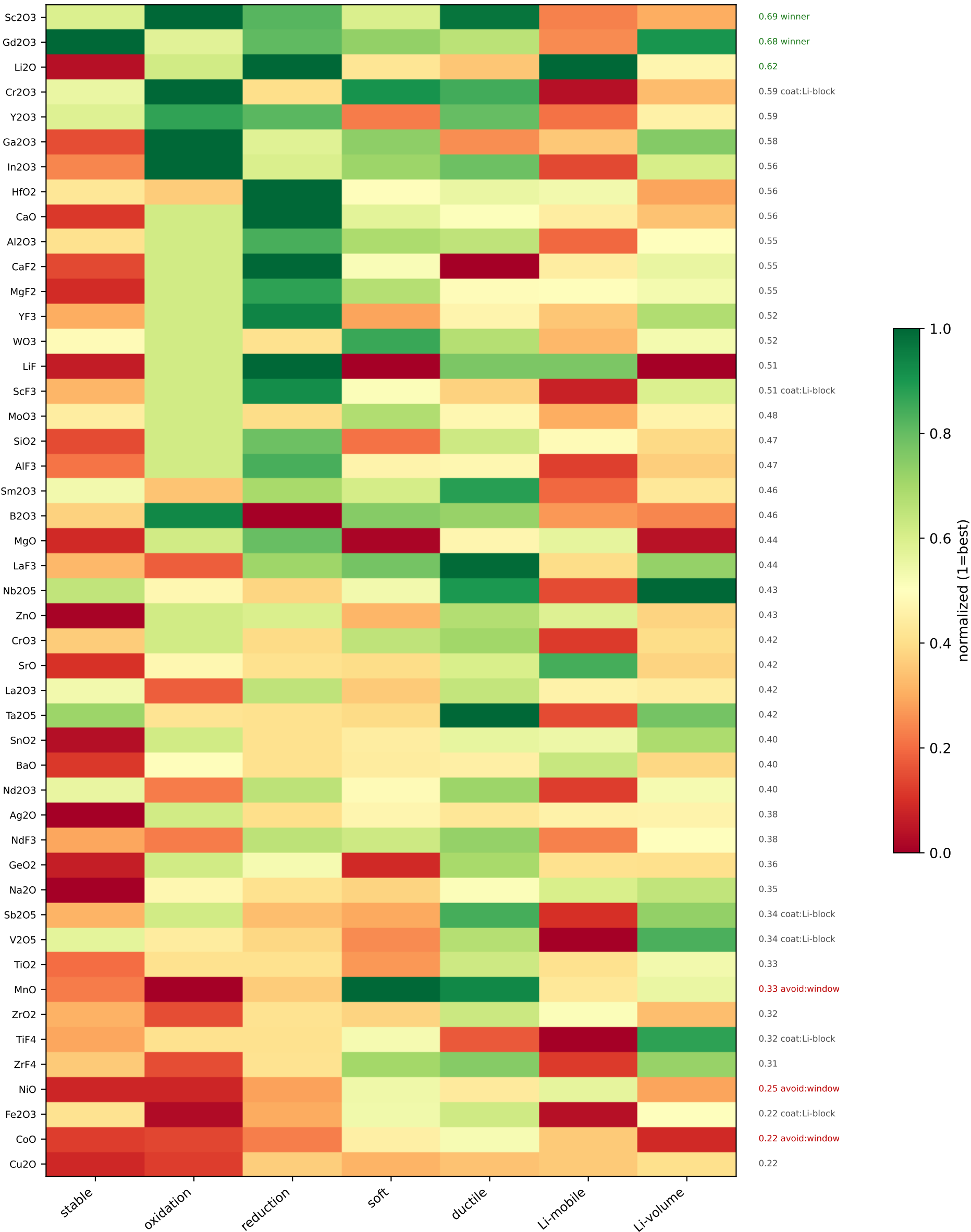
Cascade v23 MASTER SCORECARD — dopant x property (green=good), sorted by composite [x=0.25 over-doped regime; Li-mobile is high-x trend — see lit grounding]
