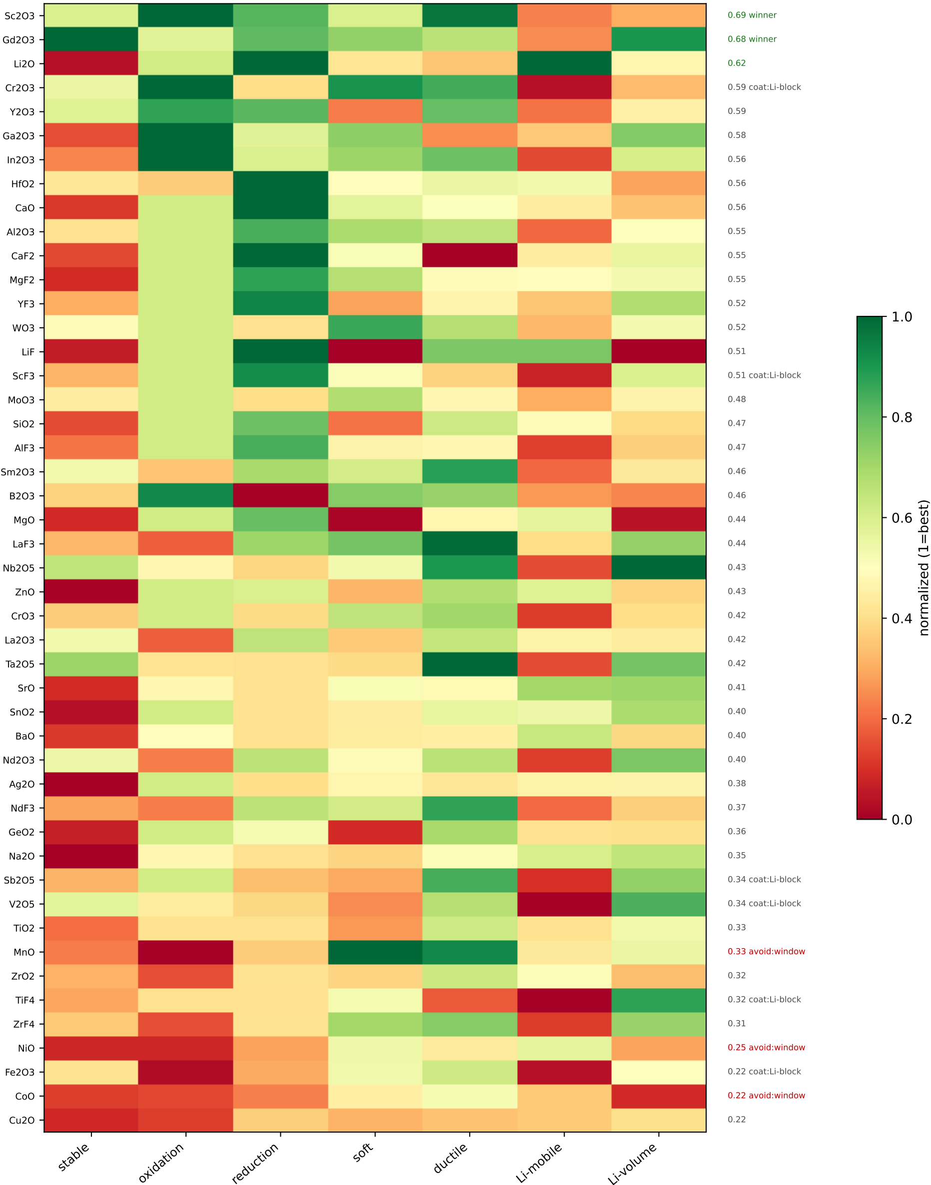
Cascade v23 MASTER SCORECARD — dopant × property (green=good), sorted by composite [x=0.25 over-doped regime; Li-mobile is high-x trend — see lit grounding]
