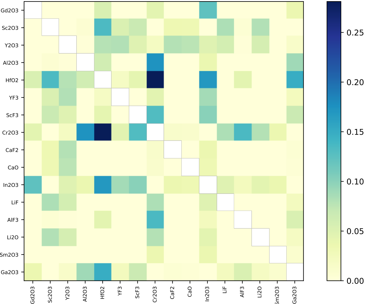
(C) Pairwise synergy among 16 best single dopants
