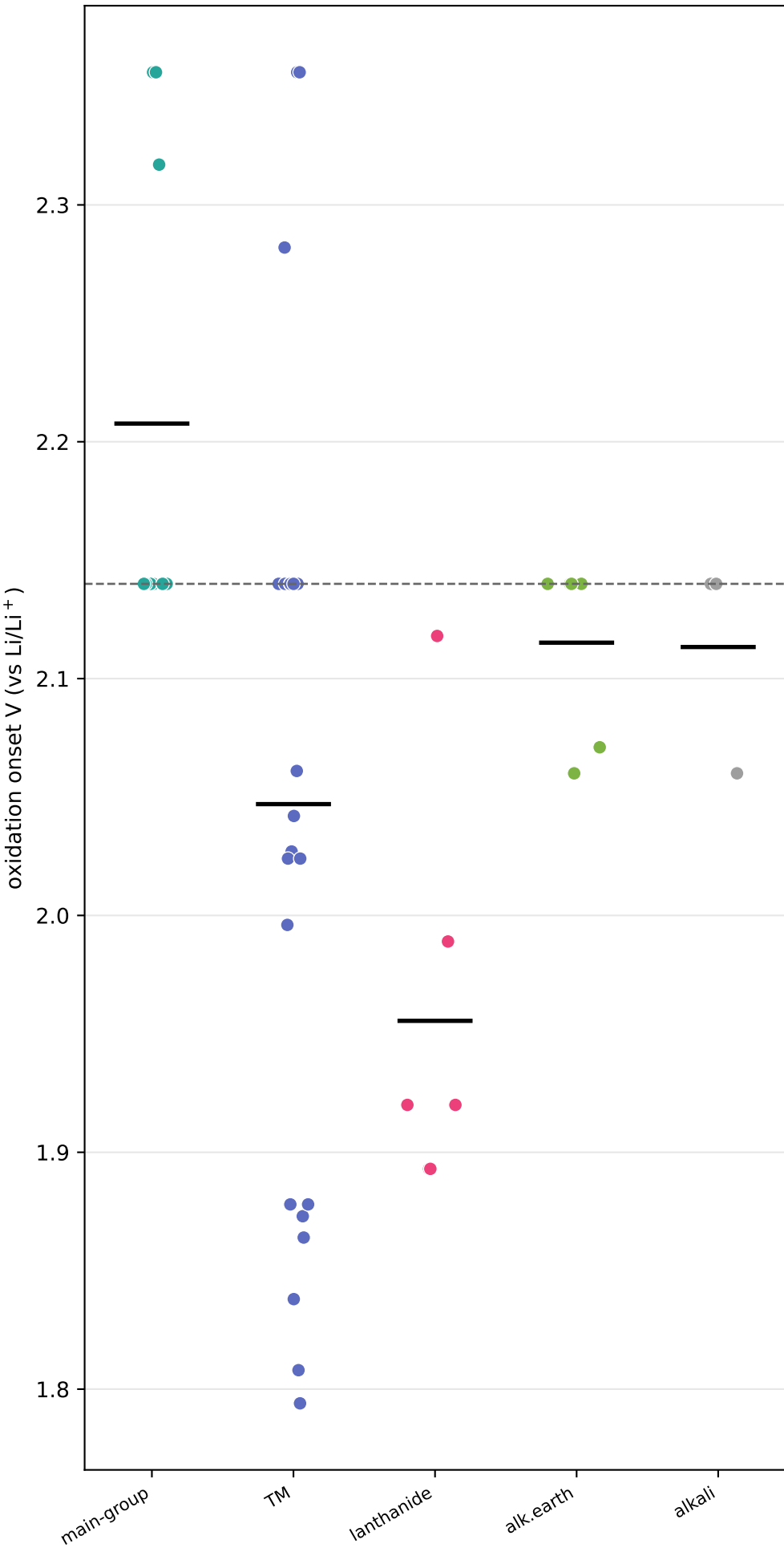
(B) Oxidation onset by cation group main-group/early-TM push it up; late-TM collapse it
