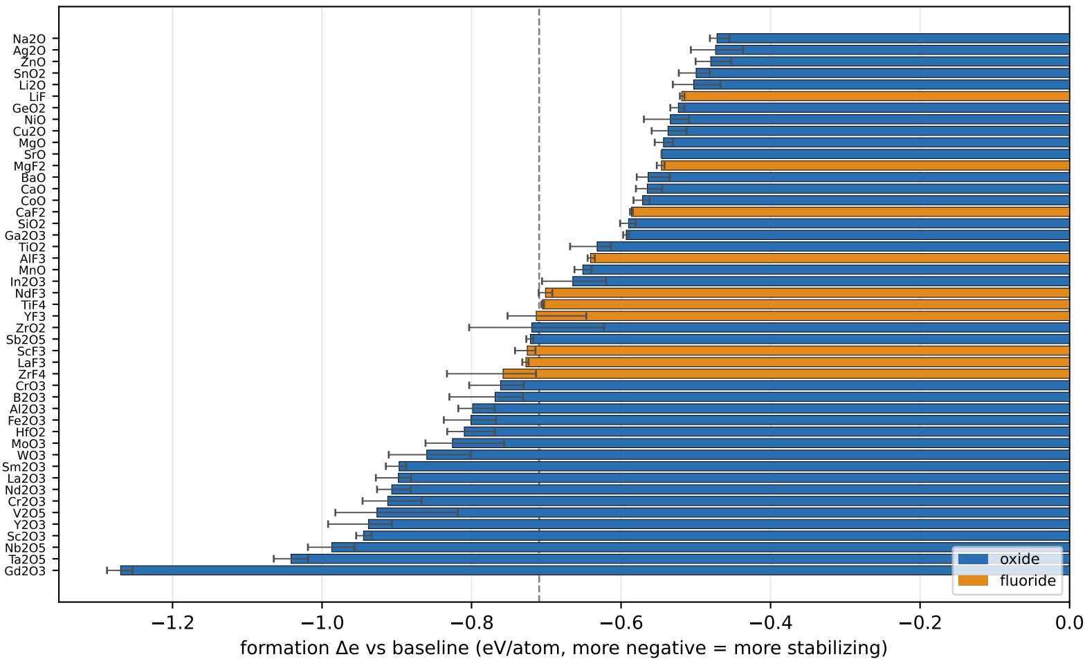
(C) Stability vs valence — higher charge cation stabilizes more
