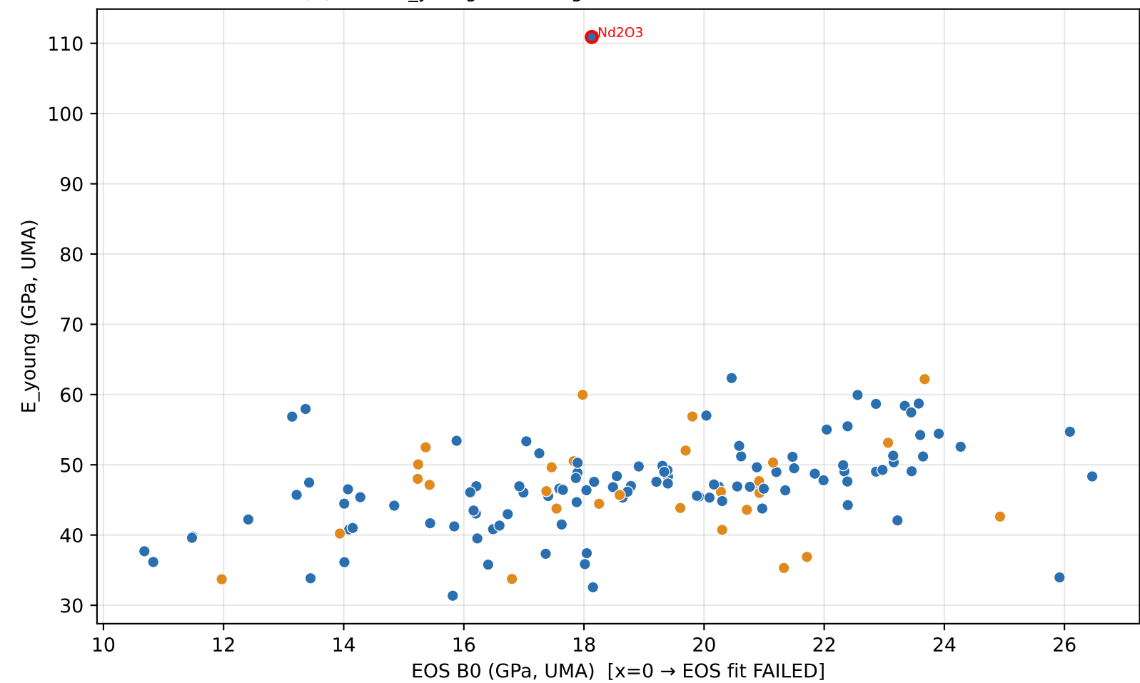
(D) B0 vs E young — red ring = elastic outlier, red x = EOS-fit fail
