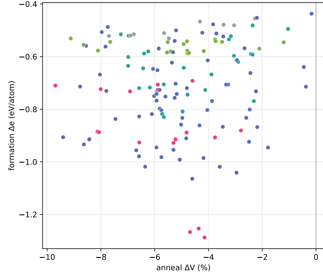
(F) Lattice strain vs stability ( |\Delta V| small = less misfit)
