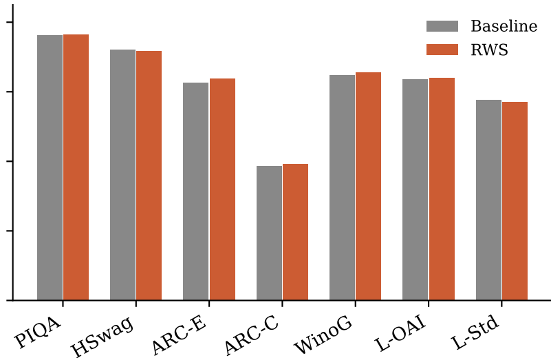
Qwen1.5-MoE @ 2.75 bit
