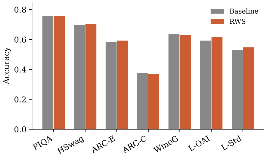
Qwen1.5-MoE @ 2.5 bit
