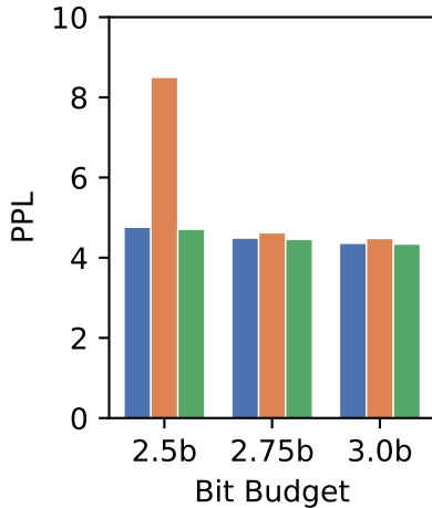
Mixtral-8x7B
