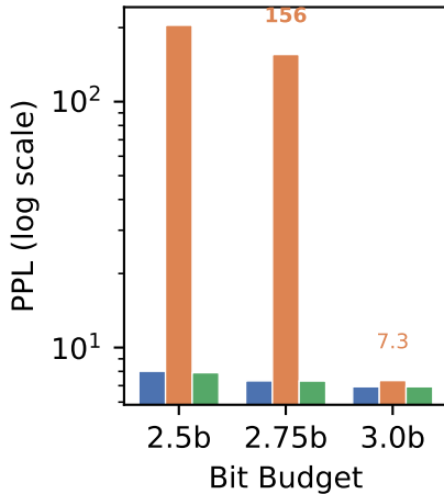
DeepSeek-MoE
