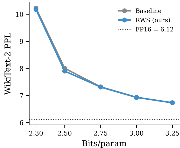
DeepSeek-MoE (RHI = 1.56)
