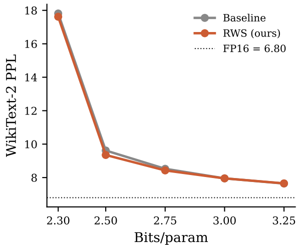
Qwen1.5-MoE (RHI = 1.84)
