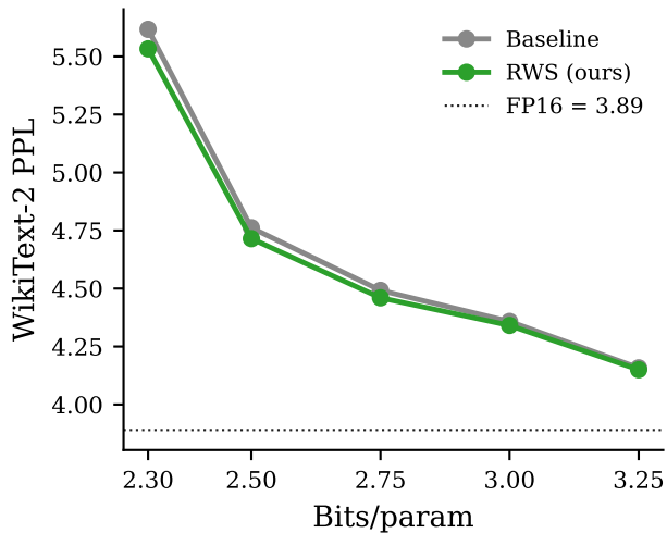
Mixtral-8x7B (RHI = 1.84)
