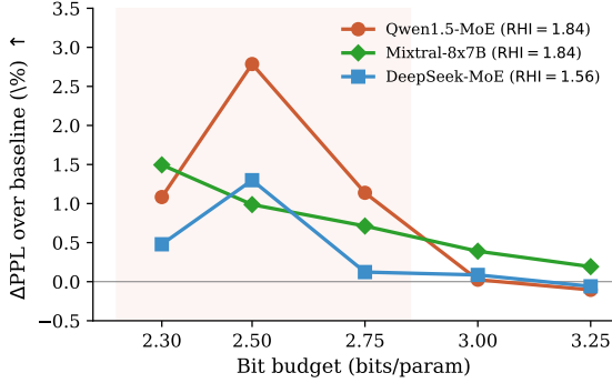
Figure 3: PPL improvement (%) vs. bit budget across three models. RWS improves over the MP baseline in the aggressive regime (shaded), with all models showing positive gains.
